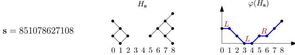
Fig. 3: An alternating word s with corresponding heap H_s , and its encoding by a walk.
