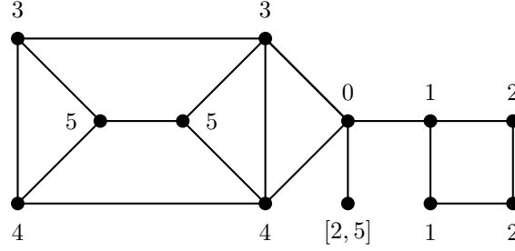
Fig. 1: A K_{2,3} -amenable graph G
