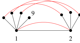
Fig. 1: The multigraph corresponding to the minimum 2-reachable sequence given in the proof of Theorem 2. All vertices except 1 and 9 have deficiency 0.
