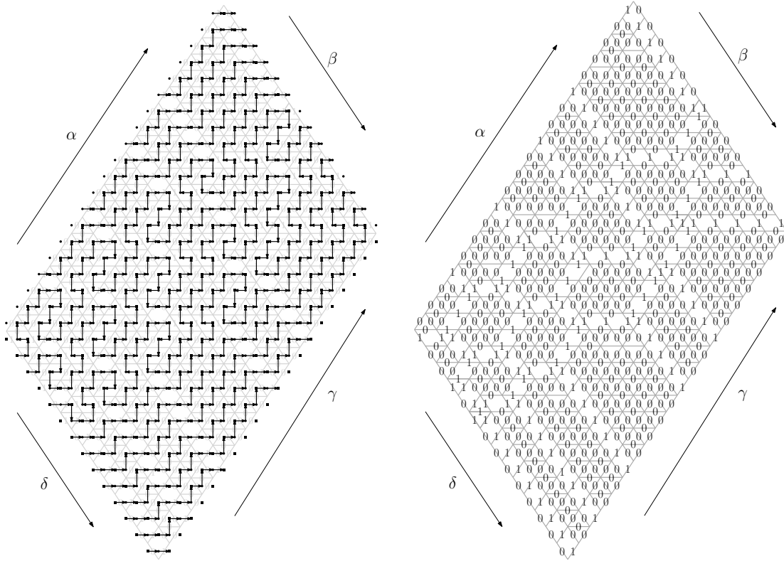
Fig. 6: An oriented RFPL and its corresponding rhomboid-shaped Knutson-Tao puzzle of size (20,14) with boundary (0001000100001001000001, 00000010001001; 10100100001001000000, 10010100000000).
