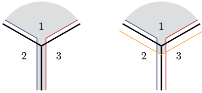
Fig. 5: Approximating neighbourhoods corresponding to a = 1 and b = 23 (on the left), respectively a = 1 and b = 123 (on the right).
