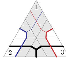
Fig. 6: An approximating neighbourhood for a = 1, b = 23 as an intersection of affine pseudohalfspaces in a blow-up of the black tropical pseudohyperplane.
