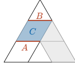
Fig. 2: The two edges A and B are mapped to the same cell under the deletion map that deletes the shaded cells.
