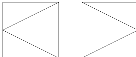
Fig. 3: Grids for unimodal arc permutations.
