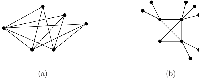
Fig. 1: (a) A complete multipartite graph K_{1,2,3} and (b) a multi-star graph K_4(0, 2, 2, 3) .
