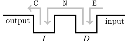
Fig. 3: The operations E, N, and C corresponding to the DI machine from Definition 2.2.
