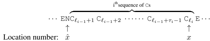
Fig. 7: An illustration of the indexing used for a word W in Observation 3.4.
